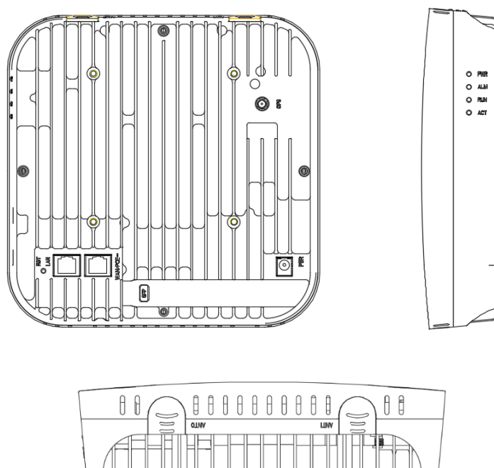
Figure 1-1 Stellar227 Appearance
